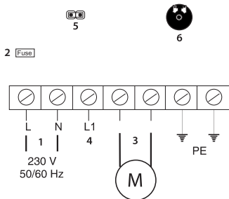
minimum speed adjustment trimmer
